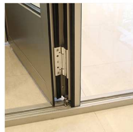
进口材质滑轨，不易生锈，耐腐蚀，使用寿命长。 Imported material slide rail, not easy to rust, corrosion resistance, long service life.
